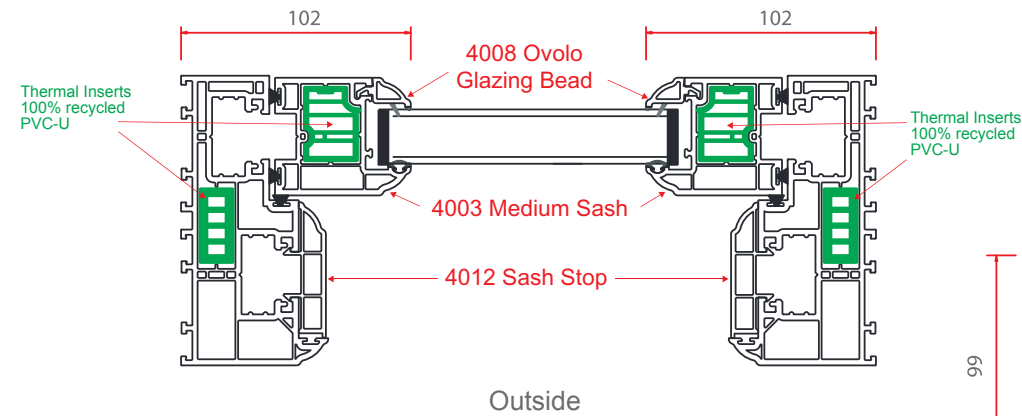
Horizontal section through bottom sash
