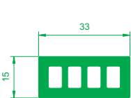
4401 Thermal Insert For 4001 Outer Frame
