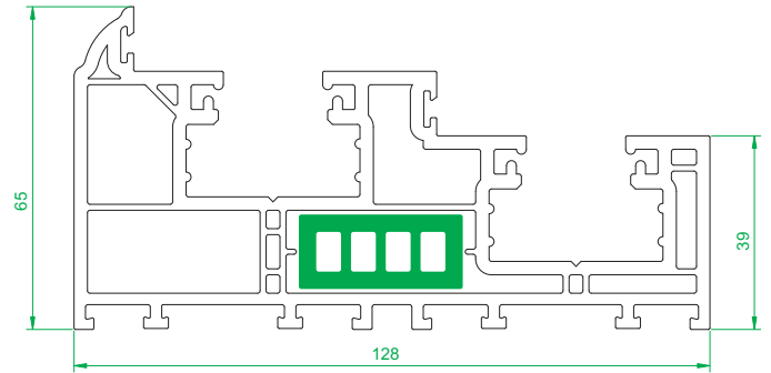
4001 Outer Frame
