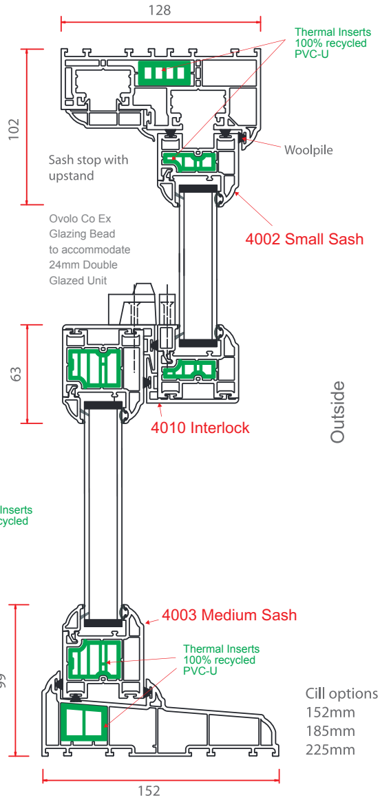
Vertical section through top sash
