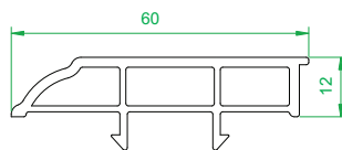
4012 Sash Stop
